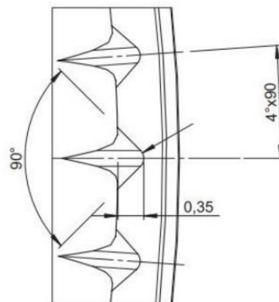
Knurls detail (20:1)
